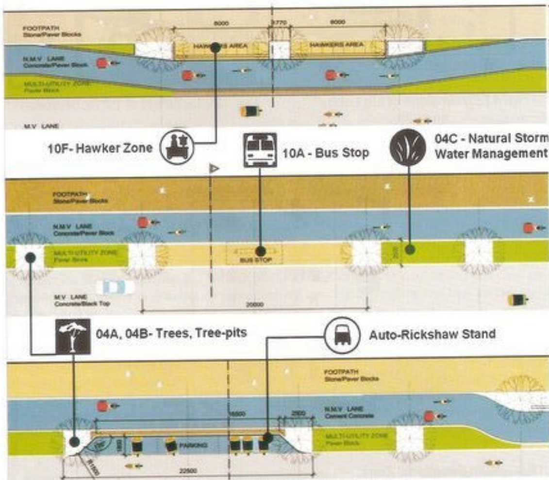
Fig. 44 Layout of Multi-Functional Zone
