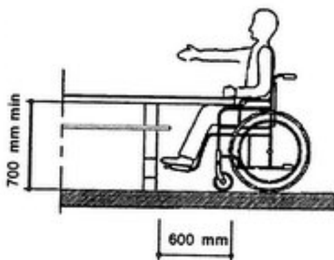
Fig. 47 Knee Clearances in Tables in Public Places
