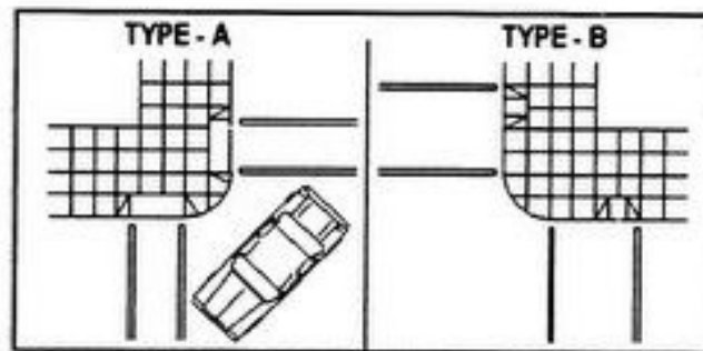
Fig. 13 Recommended Design for a Kerb Ramp
