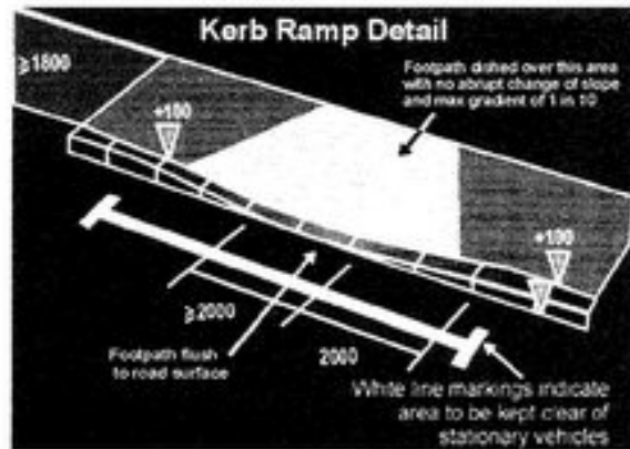
Fig. 11 Kerb Ramp Detail
