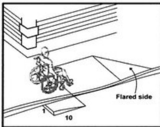
Fig. 10 Kerb Ramp
