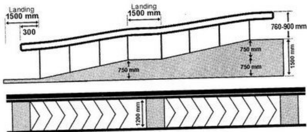
Fig. 34 Ramp Design
