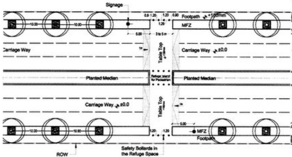
Fig. 27 Mid-Block Uncontrolled Crossing Across Two-Way Street
