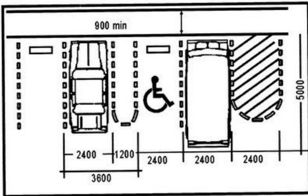
Fig. 57 Plan of Accessible Parking
