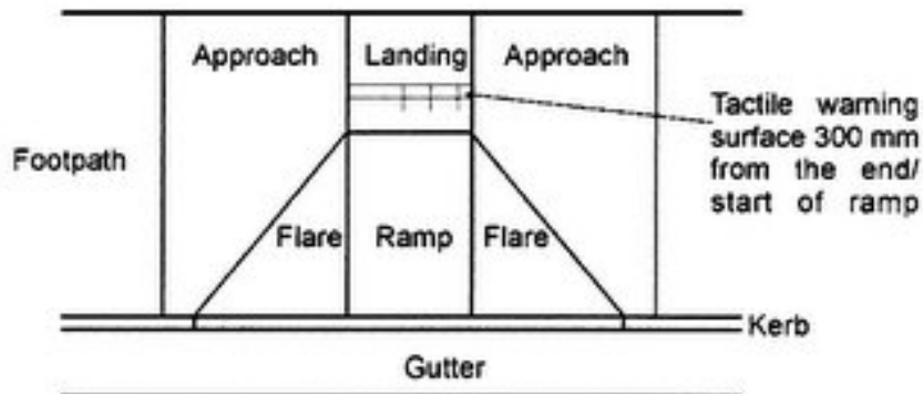
Fig. 12 Kerb Extension at Street Intersection
