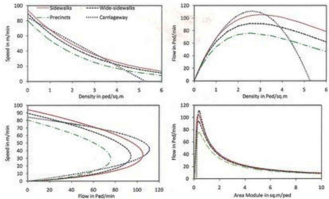
Fig. I.1: Speed –Flow-Density Relationships for Pedestrian Movements
