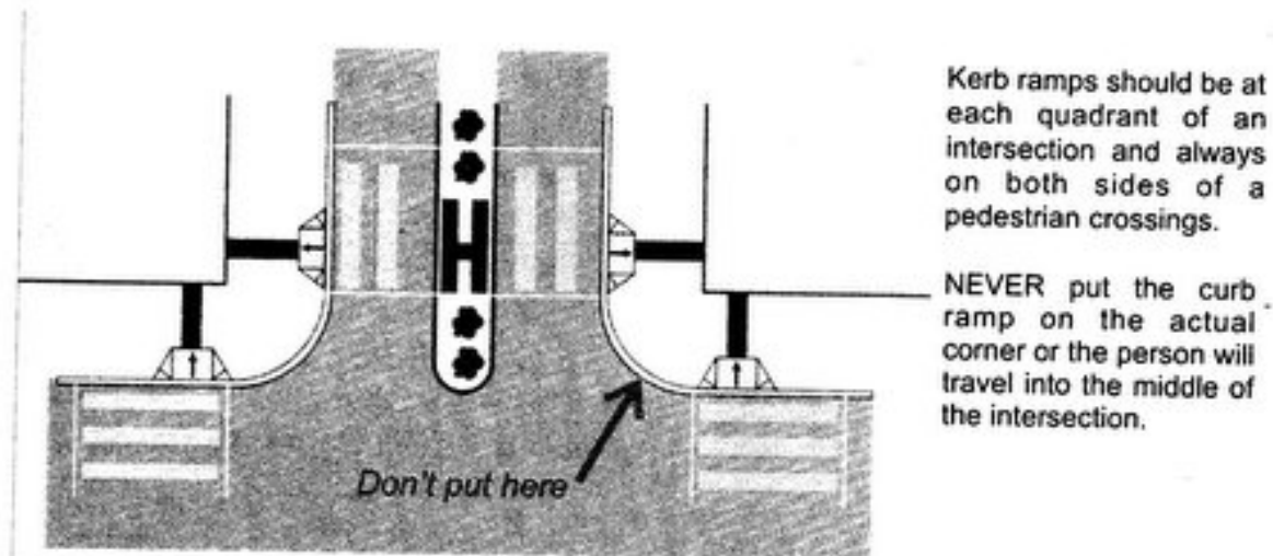
Fig. 15 Plans of Kerb Ramps at Intersections
