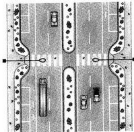
Fig. 20 Midblock Crossing Kerb Extensions
