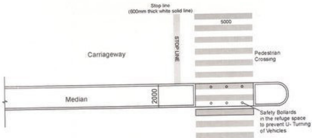
Fig. 26 Pedestrian Refuge on Two Way Road
