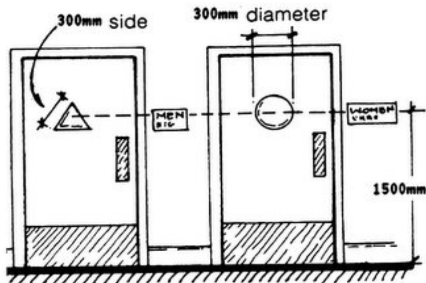
Fig. 55 Placement of Signage
