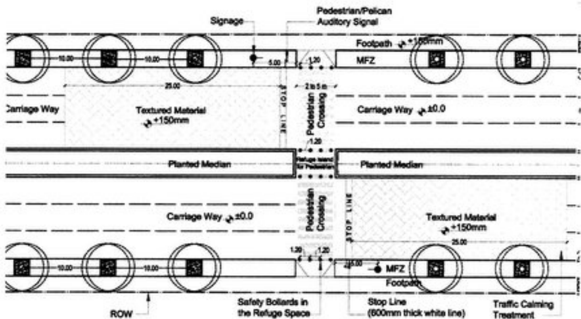
Fig. 28 Mid-Block Controlled Crossing Across Two-Way Street
