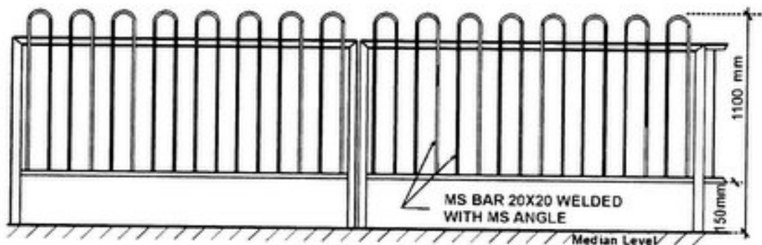
Fig. 3 Typical Design of Guard-Rail
