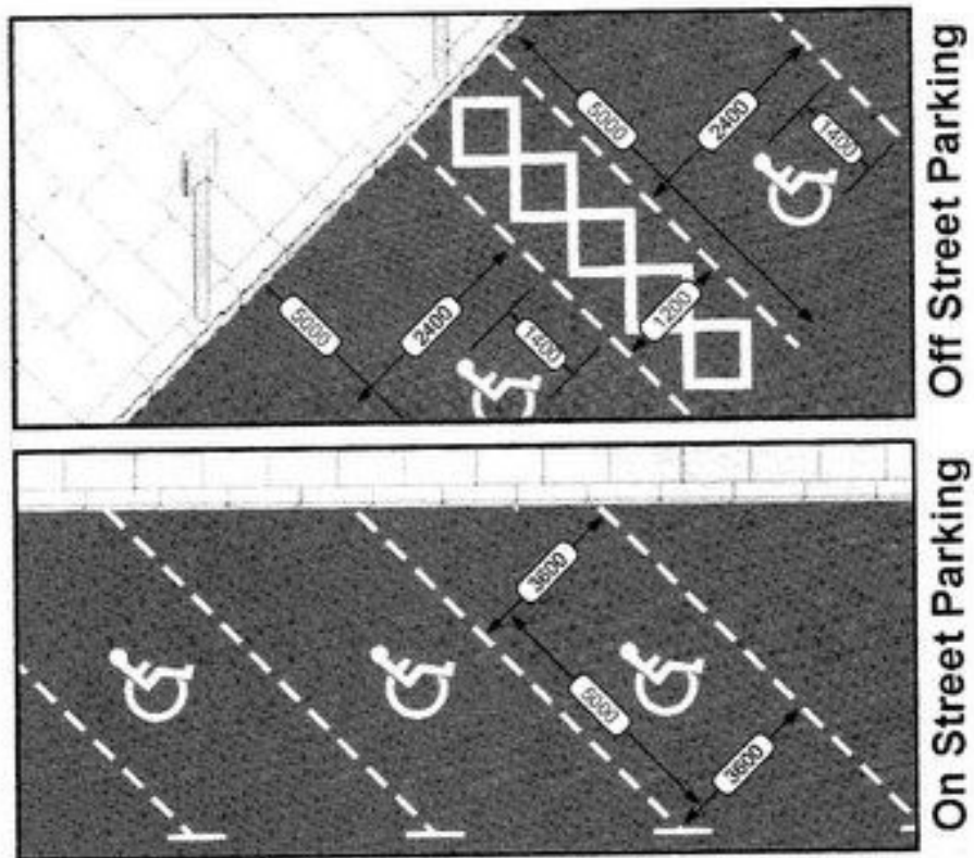
Fig. 58 Accessible Parking
