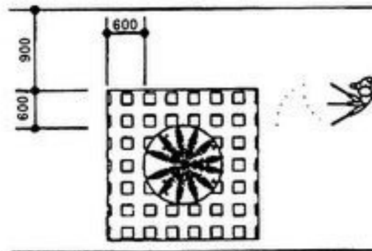
Fig. 4 Placement of Obstacles Outside Path of Travel
