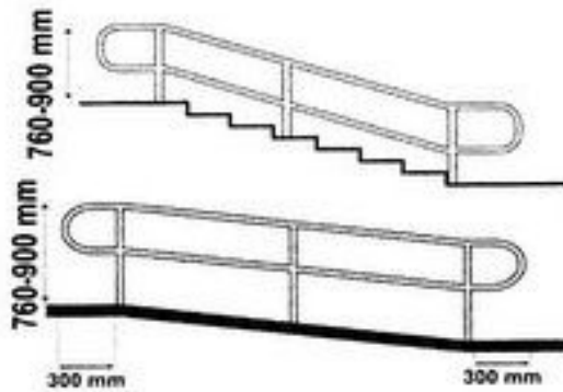
Fig. 36 Height of Handrails
