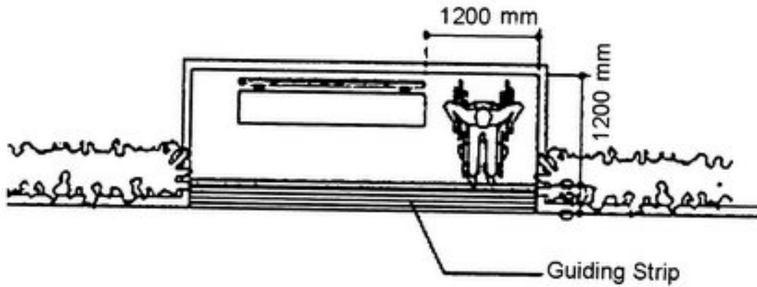
Fig. 45 Adjoining Spaces in Resting Facilities
