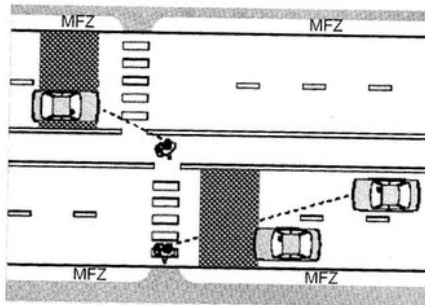
Fig. 21 A Midblock Crossing with a Median Refuge
