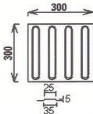
Fig. 16 Guiding Blocks
