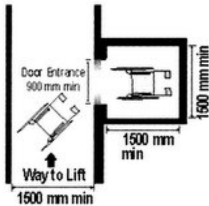
Fig. 41 Dimensions of Lift Lobby and Lift
