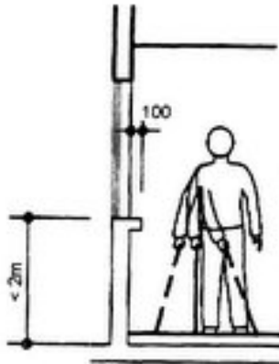
Fig. 7 Protruding Obstacles Placed in a Niche
