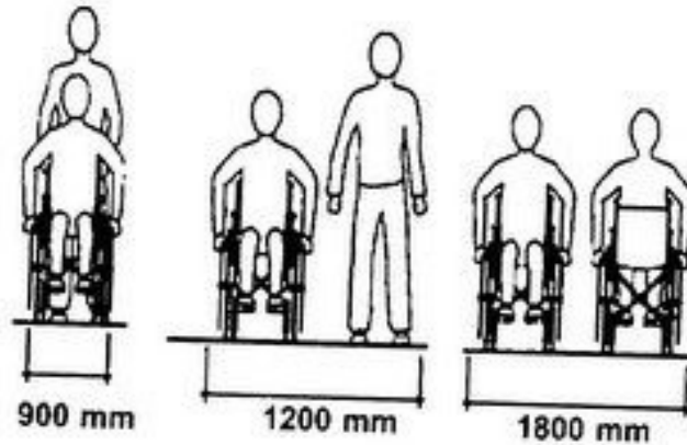
Fig. 2 Minimum Width of a Clear Footpath
