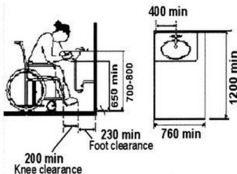
Fig. 53 Washbasin Standards
