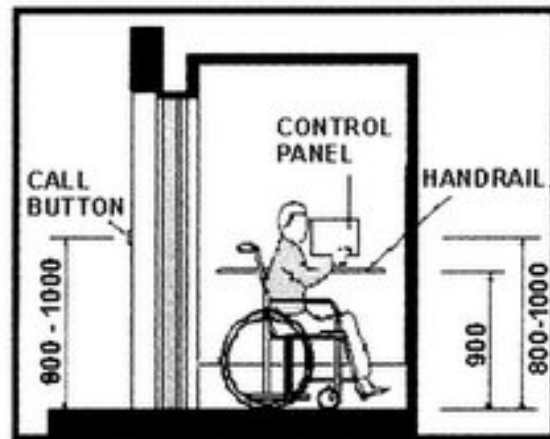
Fig. 42 Placement of Lift Accessories
