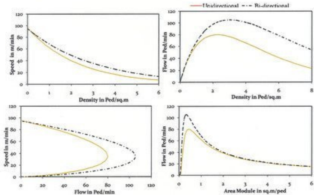
Fig. I.2: Speed-Flow-Density Relationships for Directional Movements
