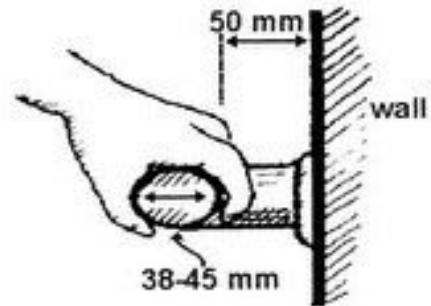
Fig. 37 Knuckle Space of Handrails
