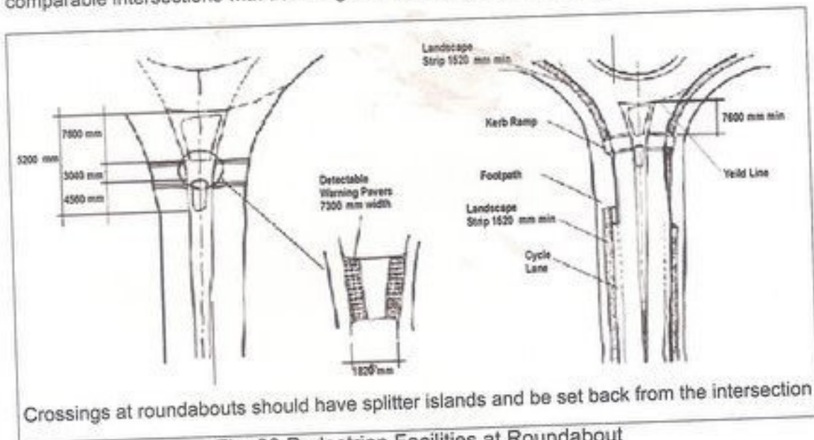
Fig. 30 Pedestrian Facilities at Roundabout
