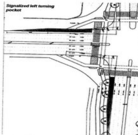
Fig. 9 Signalised Left Turning Pocket
