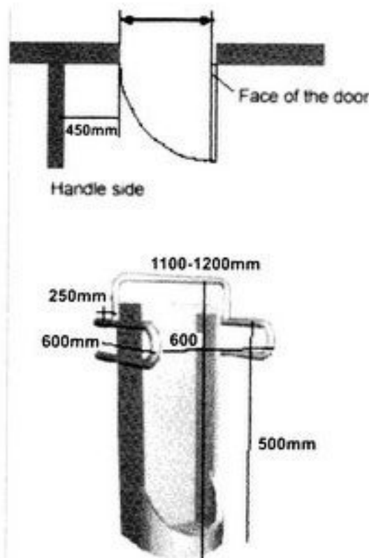
Fig. 56 Urinal with Chest Support Grab Bar
