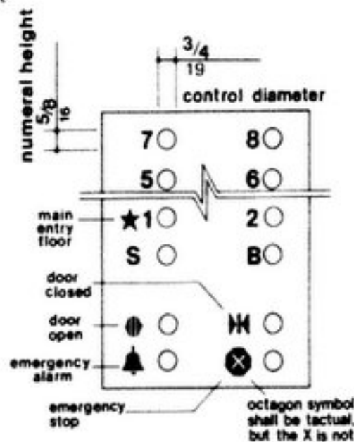
Fig. 43 Layout of Lift Control Panel
