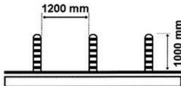
Fig. 49 Height and Gap Between Bollards
