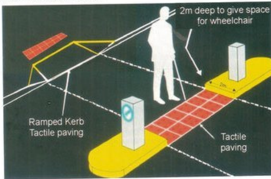
Fig. 25 Pedestrian Refuge on Two Way Road
