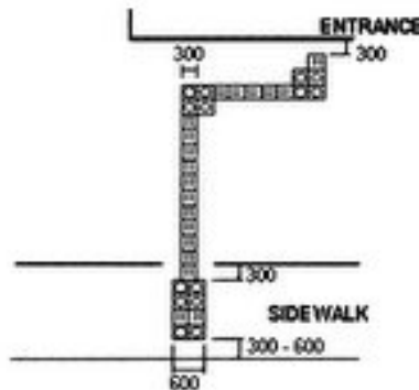
Fig. 18 Configuration of Floor Tactile Paving
