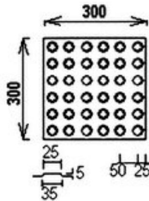
Fig. 17 Warning Blocks
